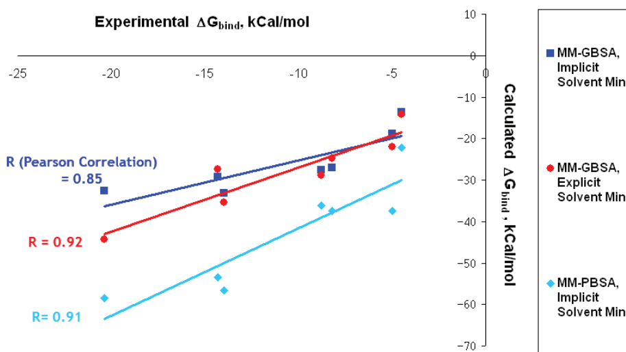
Physics-based scoring of biotin analogs (docked to avidin) using different solvation models.
