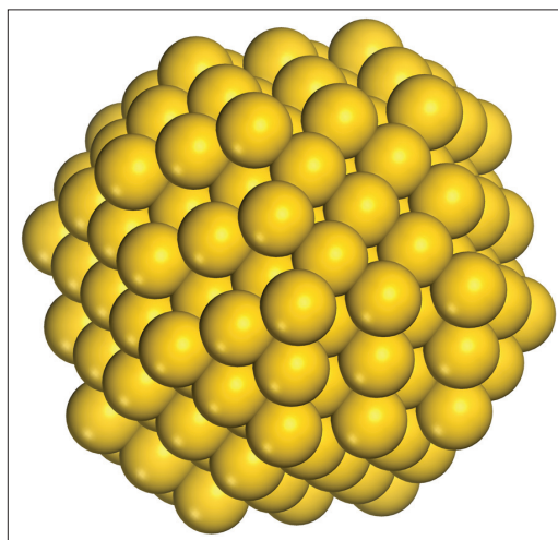
GULP geometry optimization and dynamics can be used to study the stability of clusters such as the gold nanocluster above.
