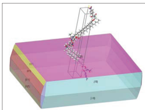
The predicted crystal morphology of the most stable polymorph of CAPP (chloramphenicol-3-palmitate).
