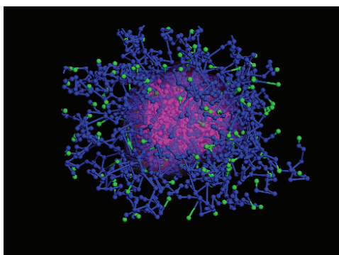
Figure 3. Surfactant micelle in aqueous solution (water not shown).
