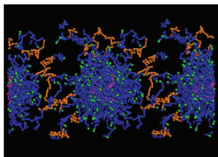
Figure 6. Snapshot of the system containing non-ionic surfactant, hydrophobic drug and non-ionic polymeric surfactant in aqueous solution (water not shown).
