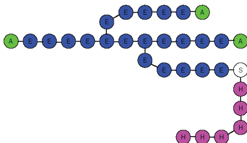
Figure 2. Coarse-grained model of the non-ionic surfactant molecule.
